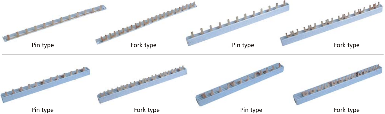
LT-12 2x16mm 2 LT-25 2x25mm 2 LT-35 2x35mm 2 LT-50 2x50mm 2 LT-70 2x70mm 2 LT-95 2x95mm 2 LT-120 2x120mm 2
